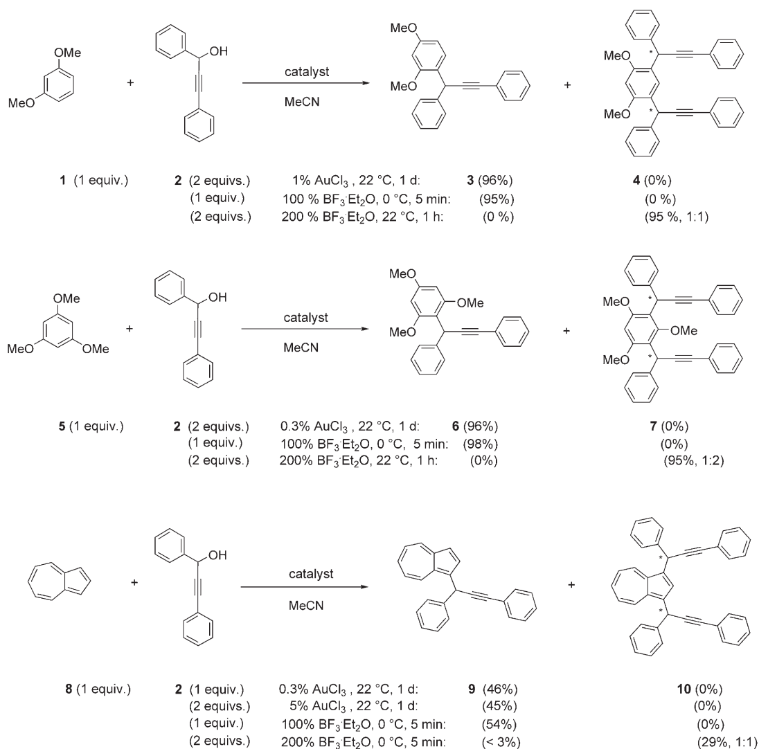
Scheme 1. Propargylation of electron-rich arenes.
