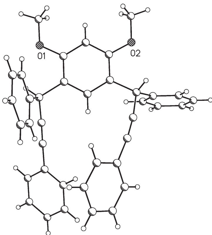
Figure 1. Molecular structure of the SS -enantiomer of 4 , hydrogen atoms omitted for the sake of clarity.
