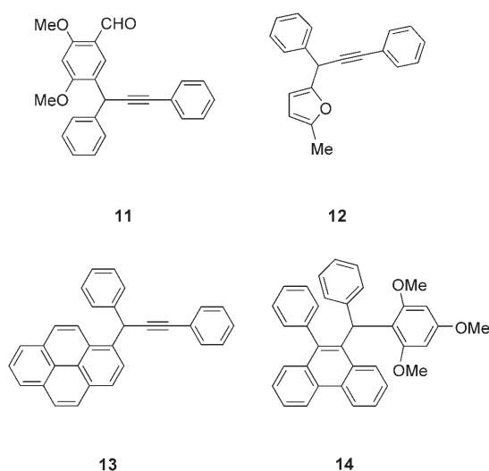
Scheme 2. Additional products from propargylation reactions and further transformations.
