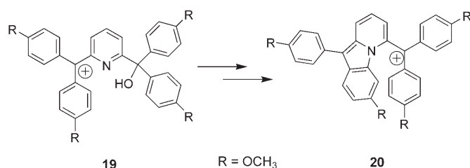
Scheme 4. Reactive intermediates of the formation of 18 .
