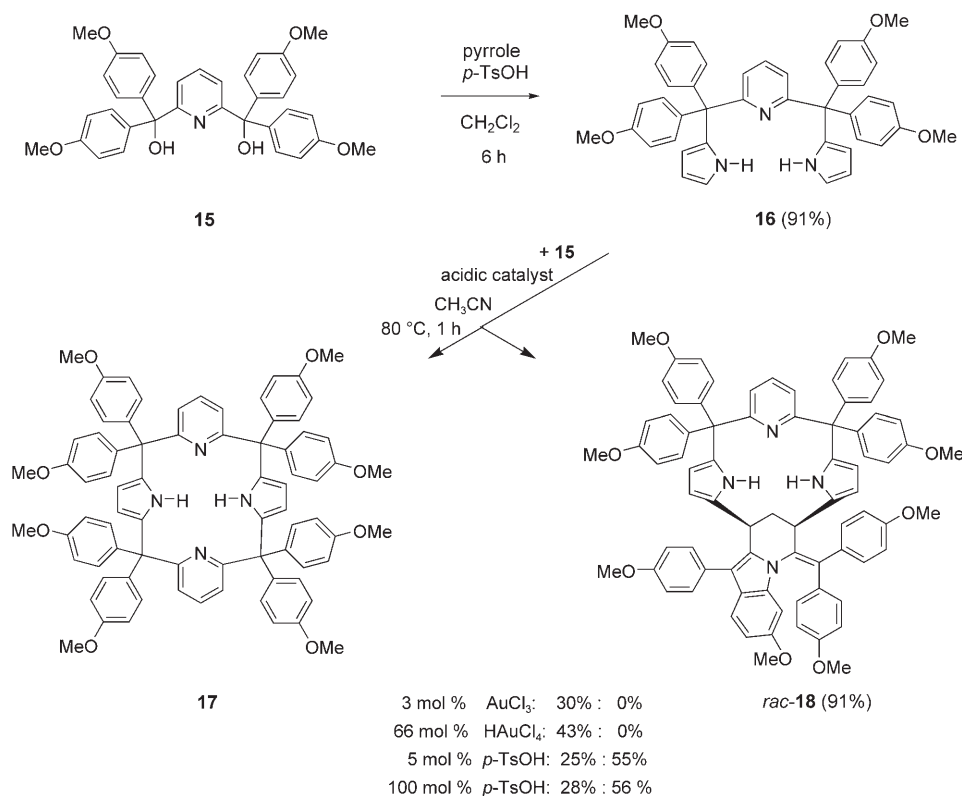
Scheme 3. Au-catalyzed macrocyclization and its acid-catalyzed competing reaction.
