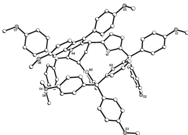
Figure 2. Molecular structure of 18 , hydrogen atoms omitted for the sake of clarity.
